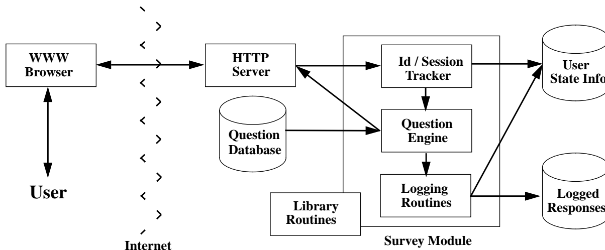
Figure 1. The above diagram overviews the architecture used for the implementation of one surveys.
